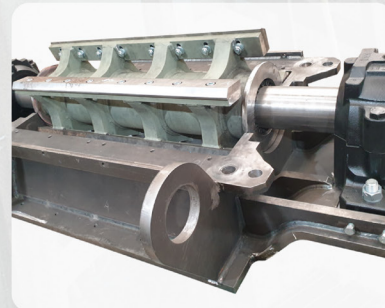
Heavy duty rotor.
